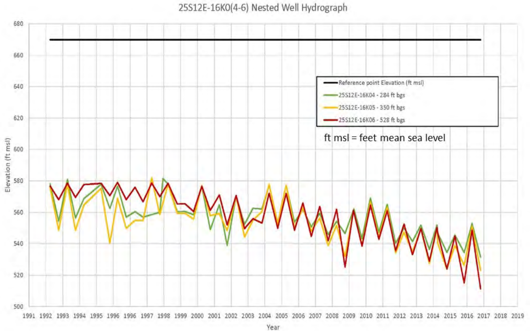
Figure 5-10. Vertical Groundwater Gradients near San Miguel
