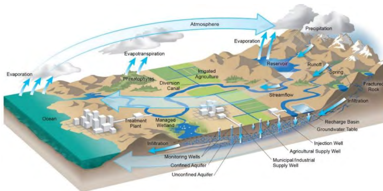
Figure 6-1. Hydrologic Cycle
