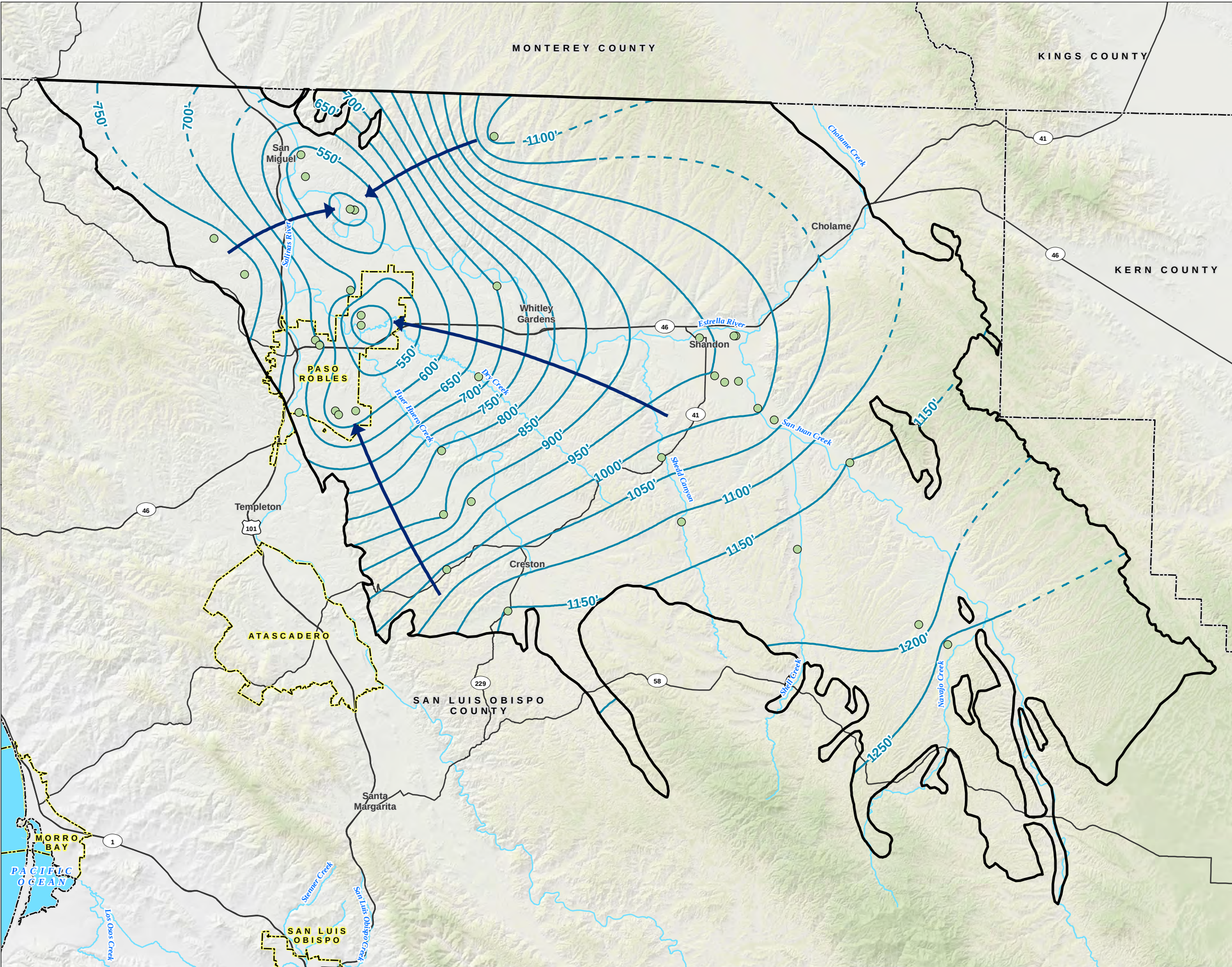
FIGURE 9 Paso Robles Formation Aquifer Fall 2019 Groundwater Elevation Contours
