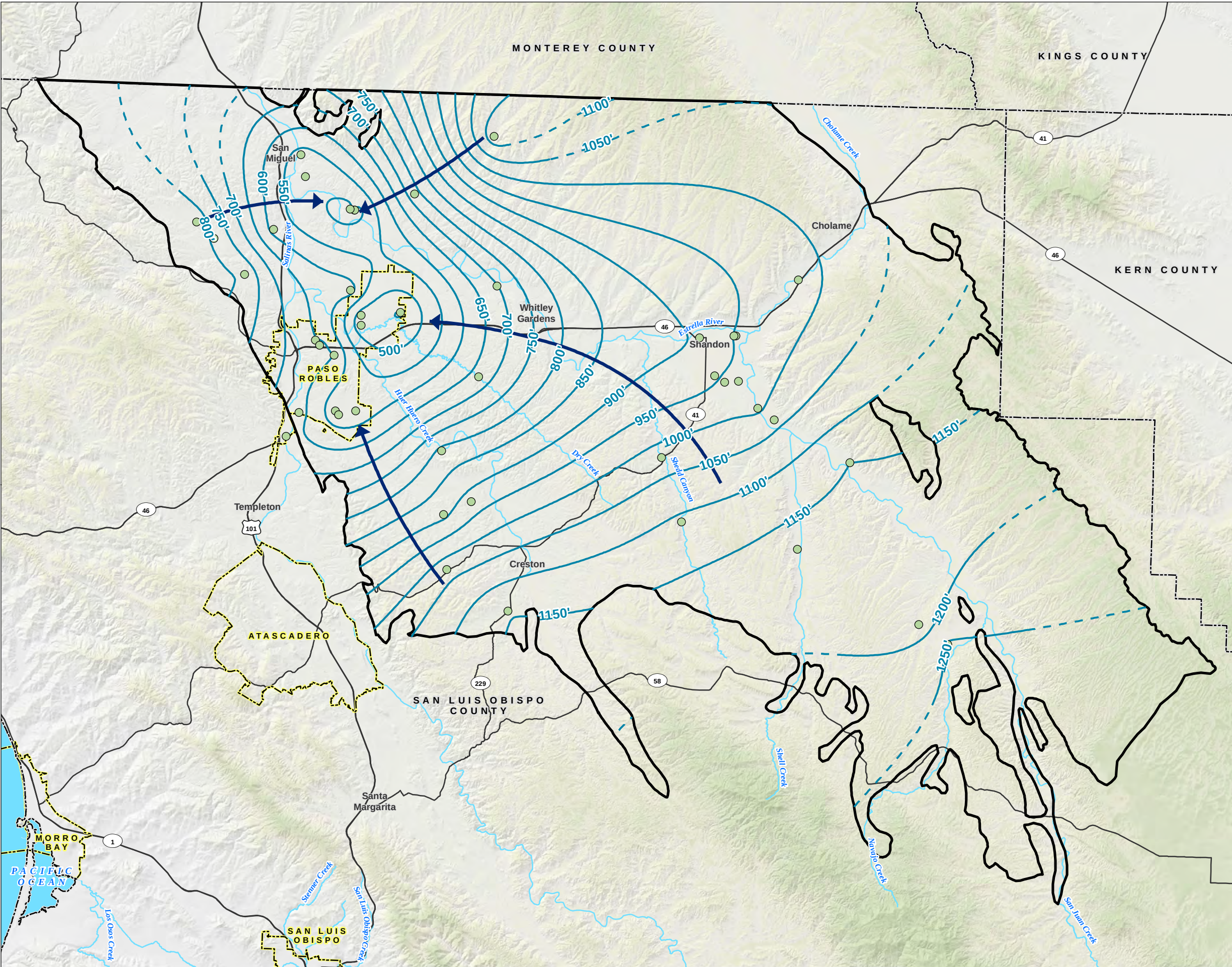
FIGURE 5 Paso Robles Formation Aquifer Fall 2017 Groundwater Elevation Contours Paso Robles Subbasin First Annual Report
