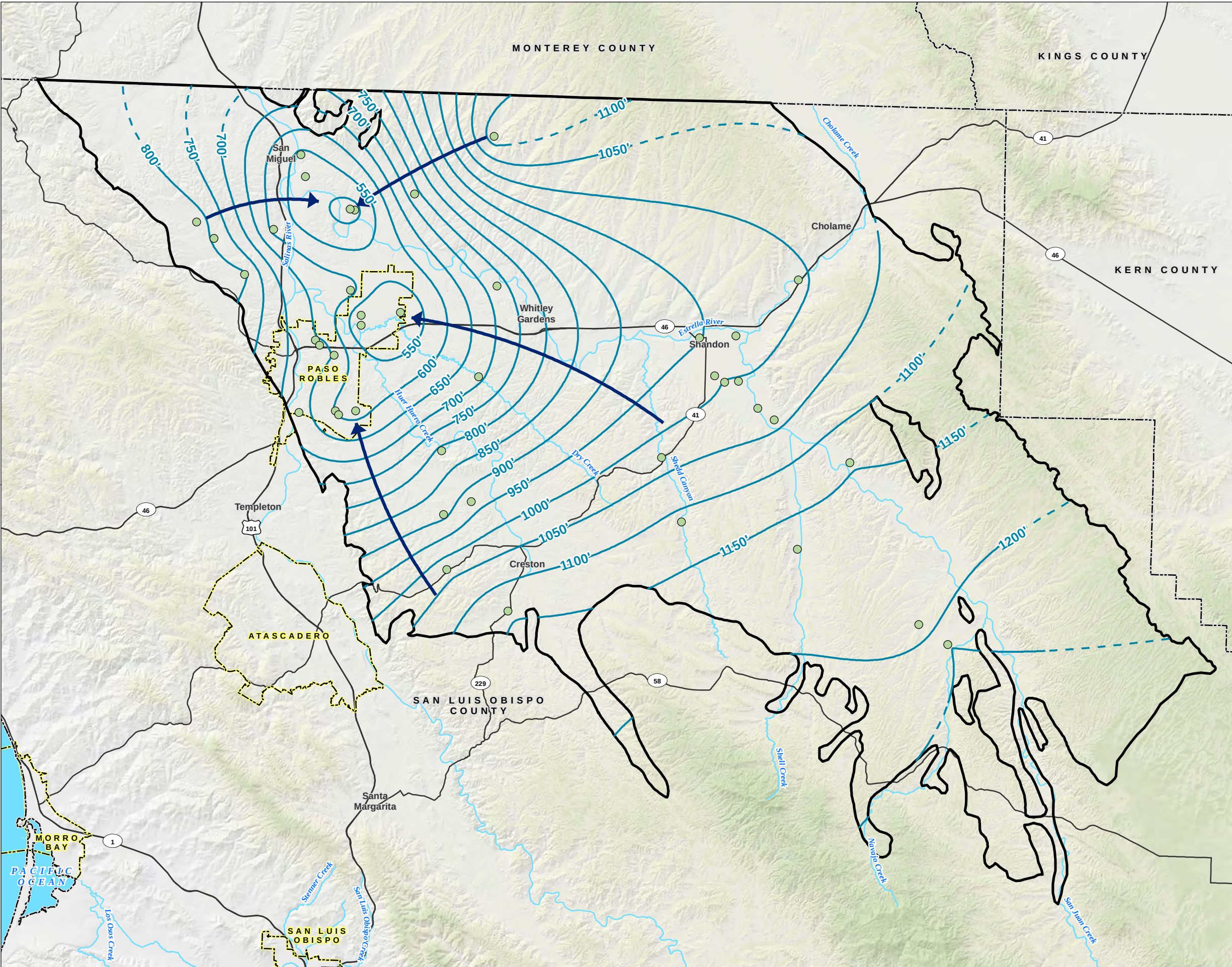
FIGURE 6 Paso Robles Formation Aquifer Spring 2018 Groundwater Elevation Contours
