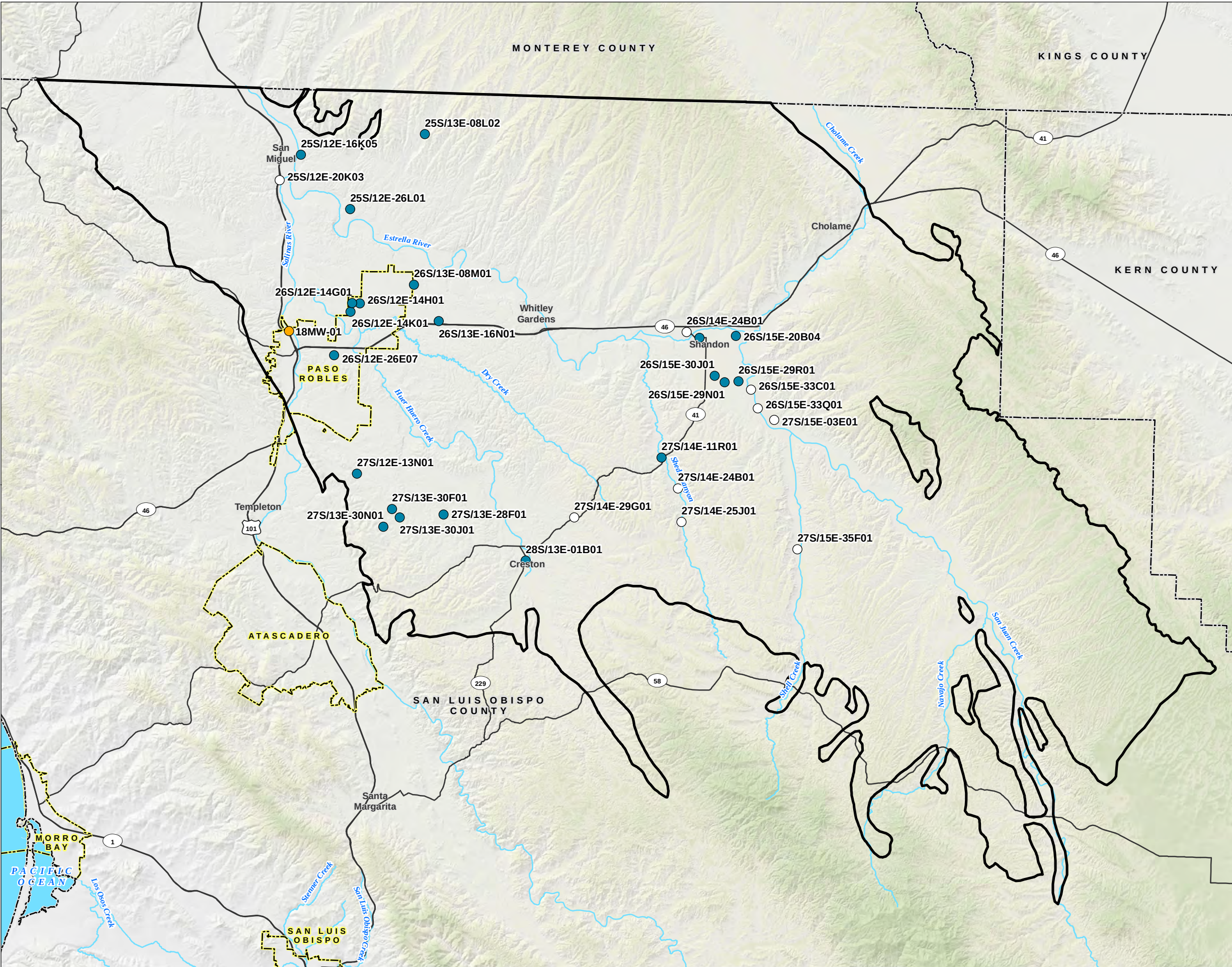
FIGURE 3 Groundwater Elevation Monitoring Well Network in the Paso Robles Subbasin
